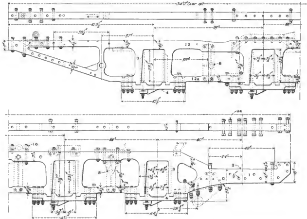
Figs. 1471-1472. Cast-Steel Frame for Consolidation (2-8-0) Locomotive. American Locomotive Co.
